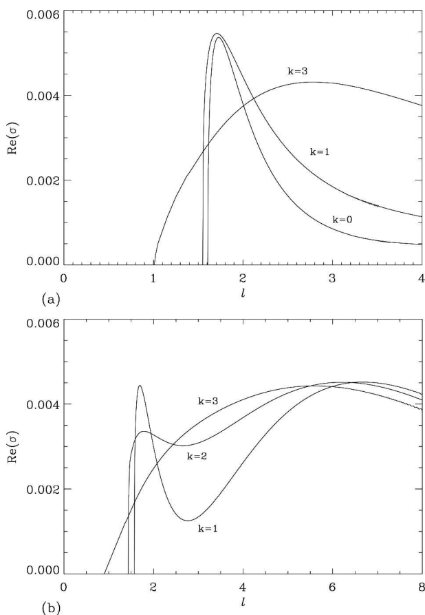
FIG. 2. Growth rate, \text{Re}(\sigma) , of the ageostrophic instability mode for \text{Ri} = 2 ( \text{Ro} = 1/\sqrt{2} ) as a function of streamwise wavenumber l for several values of cross-stream wavenumber k : (a) \lambda = 1.0 and (b) \lambda = 0.0 (the hydrostatic limit).
