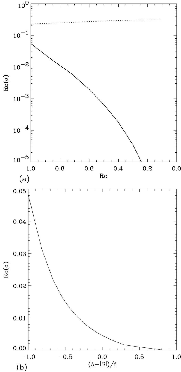
FIG. 4. Growth rates maximized over both horizontal wavenumbers for the hydrostatic regime, \lambda = 0.01 : (a) geostrophic (dots) and ageostrophic (solid) modes as a function of Ro ; (b) only the ageostrophic mode as a function of the third condition for breakdown of the balance equations, (A - S)/f .
