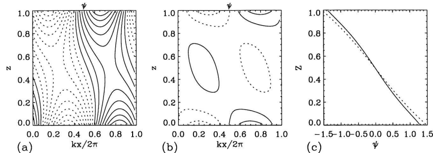
FIG. 5. (a) Streamfunction, \Psi(x, z) , for the geostrophic instability ( Ro = 1 ). (b) The unbalanced component, \Psi_{un}(x, z) , based on a total energy norm in the cost function. (c) Vertical profiles of \Psi (solid) and \Psi_{bal} (dots) at x = 0 .
