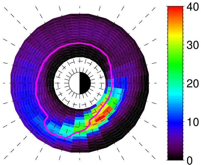
2001-06-09/20:00:00.000 Pressure, nT
