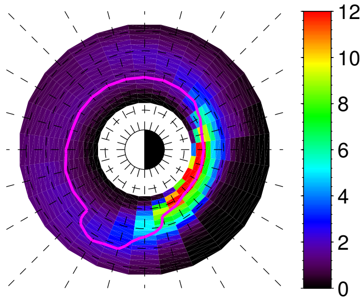
H+ density, \text{cm}^{-3}
