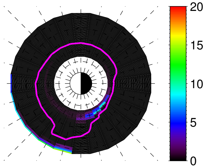
H+ band gain, dB
