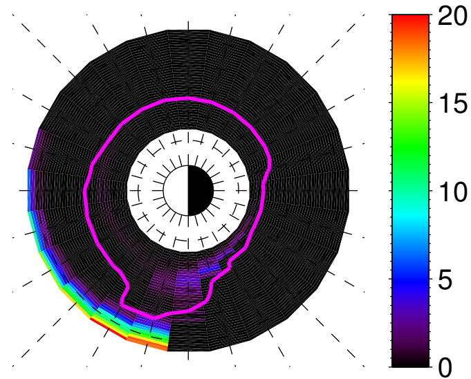
He+ band gain, dB
