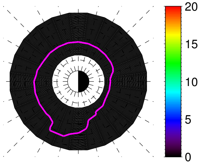
O+ band gain, dB
