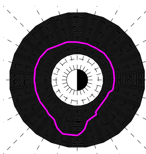
O+ band gain, dB
