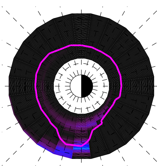
He+ band gain, dB
