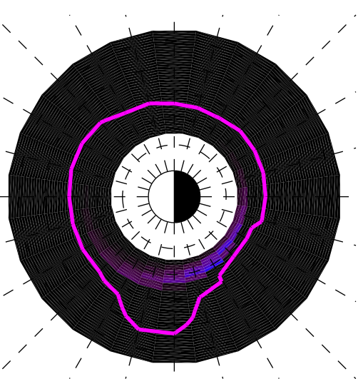
H+ band gain, dB
