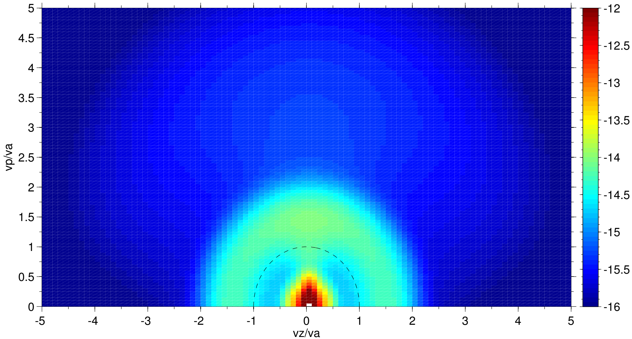
event2 m odel2 f inal:log10(PSD in s3m-6)
