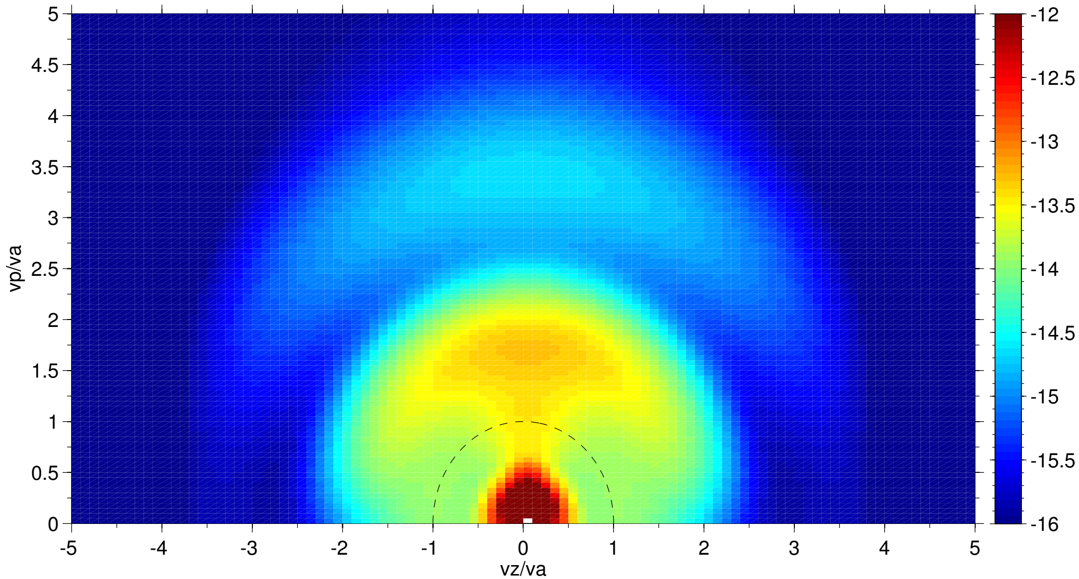
event1 m odel2 f inal:log10(PSD in s3m-6)
