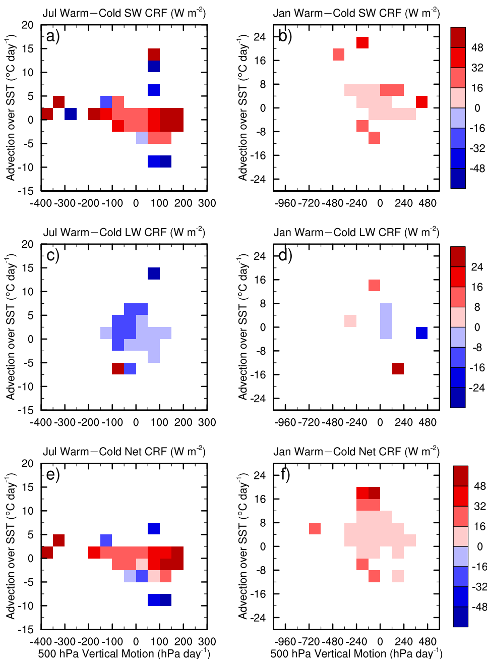
FIG. 8. Composites of the ERBE SW, LW and NET cloud radiative forcing difference between the upper (warm) and lower (cold) SST terciles for July and January during 1985-89 in \omega_{500} and advection intervals over the North Pacific ( 25-55^{\circ}N , 145-225^{\circ}E ). The magnitude of SW CRF decrease with rising temperature under most conditions of vertical velocity and SST advection (the advection of the 1000 hPa wind over the SST gradient). The cloud amount and optical thickness also decrease with rising temperature (not shown). The magnitude of LW CRF decreases, but the change in SW CRF is larger, so net CRF becomes less negative (or more positive) with warmer temperature. From Norris and Iacobellis (2005).
