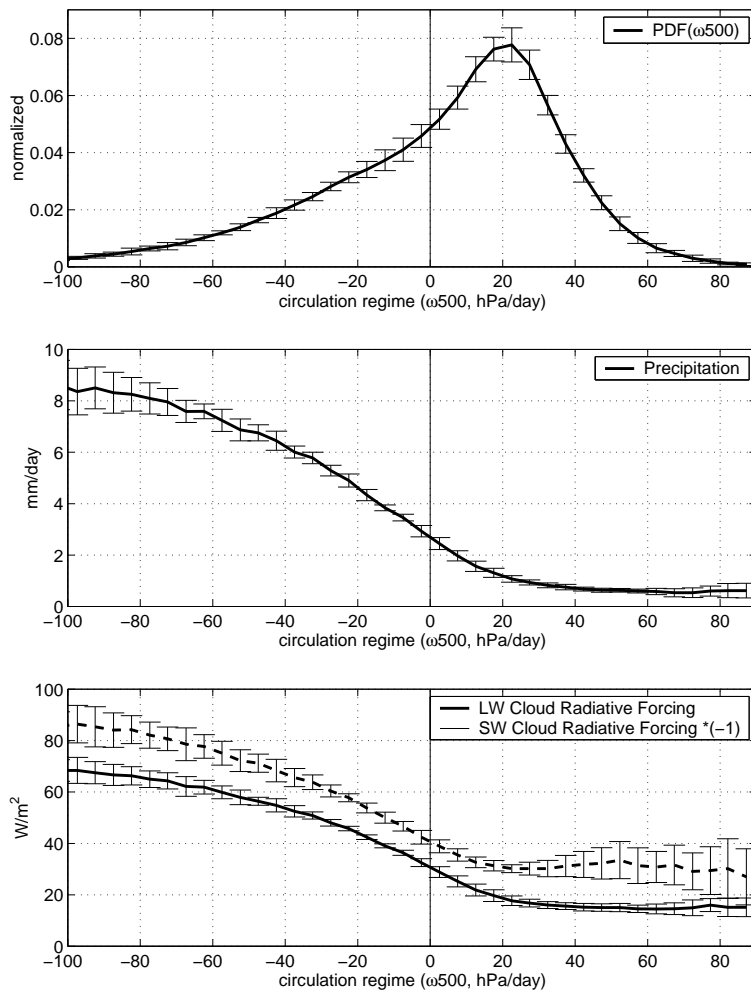
FIG. 4. (a) Probability Distribution Function P_\omega of the 500 hPa monthly-mean large-scale vertical velocity \omega_{500} in the tropics ( 30^\circ\text{S} - 30^\circ\text{N} ) derived from ERA40 meteorological reanalyses, and composite of the monthly mean (b) GPCP precipitation and (c) ERBE-derived longwave and shortwave (multiplied by -1) cloud radiative forcing in different circulation regimes defined from ERA-40 \omega_{500} over 1985-89. Vertical bars show the seasonal standard deviation within each regime. After Bony et al. (2004).
