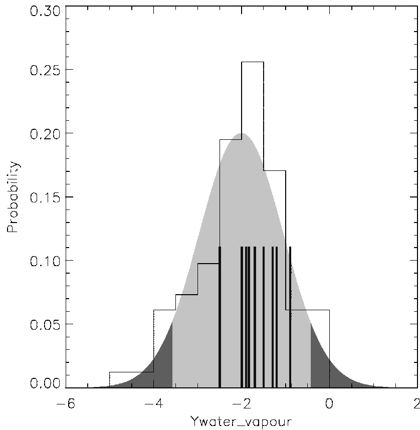
FIG. 16. Estimates of water vapor feedback parameter (in \text{Wm}^{-2}\text{K}^{-1} ) from the observations and from the HadCM3 climate model (note that the sign convention used in this figure for the definition of feedback parameters is opposite to that used in Appendix A). The histogram is computed from 82 model estimates with a bin size of 0.5 and is shown in terms of probabilities. The shaded curve is a fitted normal distribution of model estimates with the 5% and 95% represented by darker shading. Observed estimates of the water vapor feedback parameter are indicated by the vertical lines, and lie in the range 0.9 to 2.5 \text{ Wm}^{-2}\text{K}^{-1} (using the sign convention of Appendix A, i.e. positive feedbacks have positive sign). From Forster and Collins (2004).
