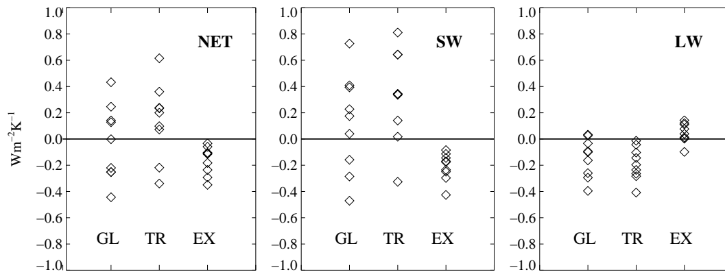
FIG. 9. Global change in the NET (left panel), SW (middle panel) and LW (right panel) cloud radiative forcing normalized by the change in global mean surface air temperature predicted by AR4 mixed-layer ocean atmosphere models in 2 \times CO_2 equilibrium experiments. For each panel, results (in Wm^{-2}K^{-1} ) are shown for global (GL), tropical ( 30^{\circ}S-30^{\circ}N , TR) and extra-tropical (EX) areas. The intermodel spread of the global CRF response to climate warming primarily arises from different model predictions of the change in tropical SW CRF. Adapted from Webb et al. (2005).
