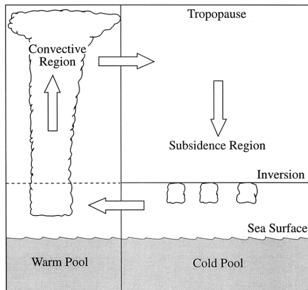
FIG. 3. Two conceptual representations of the relationship between cloudiness and large-scale atmospheric circulation in the tropics: (a) Structure of the tropical atmosphere, showing the various regimes, approximately as a function of sea surface temperature (decreasing from left to right) or mean large-scale vertical velocity in the mid-troposphere (from mean ascending motions on the left to large-scale sinking motions on the right). From Emanuel (1994). (b) Two-box model of the tropics used by Larson et al. (1999). The warm pool has high convective clouds and the cold pool has boundary layer clouds. Air is rising in the warm pool and sinking across the inversion in the cold pool.
