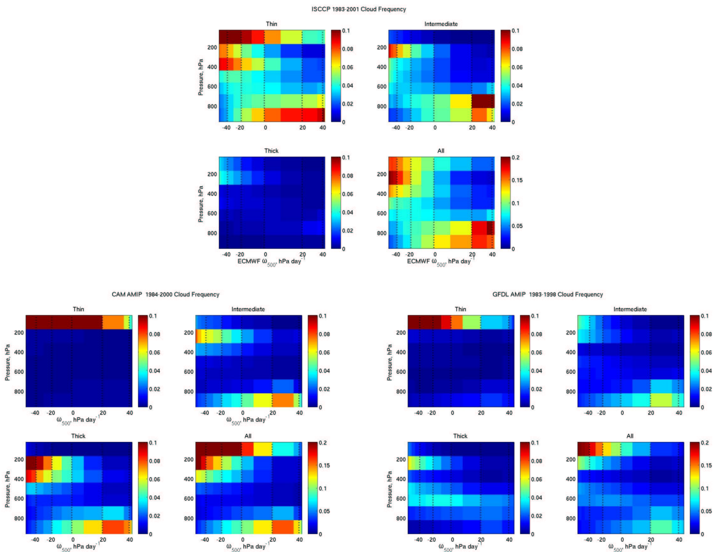
FIG. 11. Upper panel: ISCCP monthly mean cloud frequency sorted using the \omega_{500} from ECMWF analysis, and divided into ISCCP cloud thickness categories: (a) thin ( 0.1 \leq \tau \leq 3.6 ), (b) intermediate ( 3.6 \leq \tau \leq 23 ), (c) thick ( \tau \geq 23 ), and (d) all optical depths. Bottom panels: Monthly mean cloud frequency from the ISCCP simulator for an AMIP simulation of (Left) NCAR CAM 3.0 and (Right) GFDL AM2.12b climate models over the period 1984-2000, sorted by \omega_{500} and using similar thickness categories. From Wyant et al. (2005).
