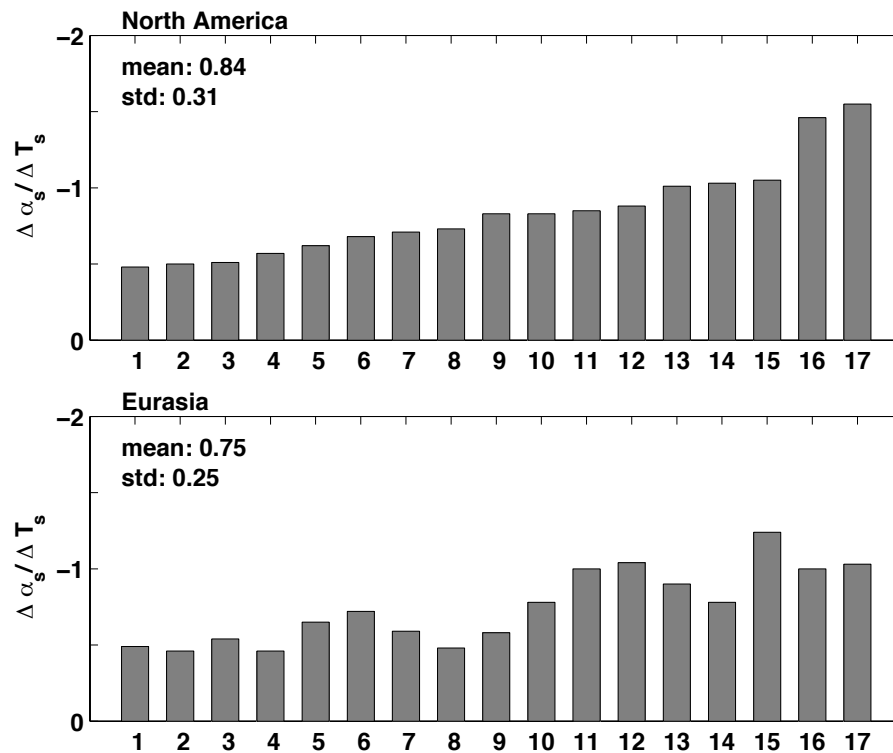
FIG. 19. The externally-forced change in springtime surface albedo (%) in snow-covered regions in the transient climate change experiments of the AR4 of the IPCC, divided by the change in springtime surface air temperature (deg C) in these experiments, a measure of the surface component of simulated springtime snow albedo feedback. The top panel is for the North American land mass, the bottom panel for the Eurasian land mass. There are 17 transient climate change experiments, each consisting of a GCM forced by observed changes and future projections of greenhouse gases and other forcing agents. The change in area-mean surface albedo (surface air temperature) is defined as the difference between area-mean surface albedo (surface air temperature) averaged over the 22 nd century of the simulations and the area-mean surface albedo (surface air temperature) averaged over the 20 th century of the simulations. Values of surface albedo were weighted by climatological incoming solar radiation at the surface in the climate of the 20th century prior to area averaging. The top panel was ordered by increasing feedback strength, and this order was preserved in the bottom panel. The fact that the feedback strength also generally increases in the bottom panel suggests a consistency in the strength of the feedback between the land masses within any single model. From Qu and Hall (2005b).
