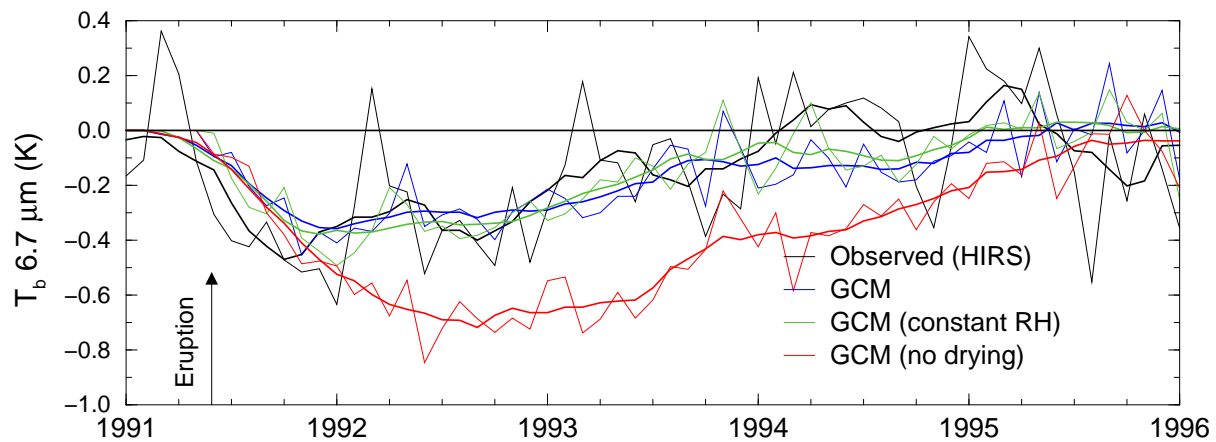
FIG. 15. Comparison of the observed (black) and GCM-simulated (blue) changes in global-mean (90S-90N) 6.7 \mu\text{m} brightness temperature ( T_b ). The observed anomalies are computed with respect to a 1979 to 1990 base climatology and expressed relative to their pre-eruption (January to May 1991) value. The GCM-simulated anomalies are computed as the ensemble-mean difference (Pinatubo - control) from three pairs of GCM simulations. The green curve depicts the GCM-simulated T_b computed under the assumption of a constant relative humidity change. The red curve depicts the GCM-simulated T_b computed under the assumption of a constant, seasonally varying water vapor mixing ratio (i.e., no drying of the upper troposphere). The thick lines depict the 7-month running mean of each time series. From Soden et al. (2002).
