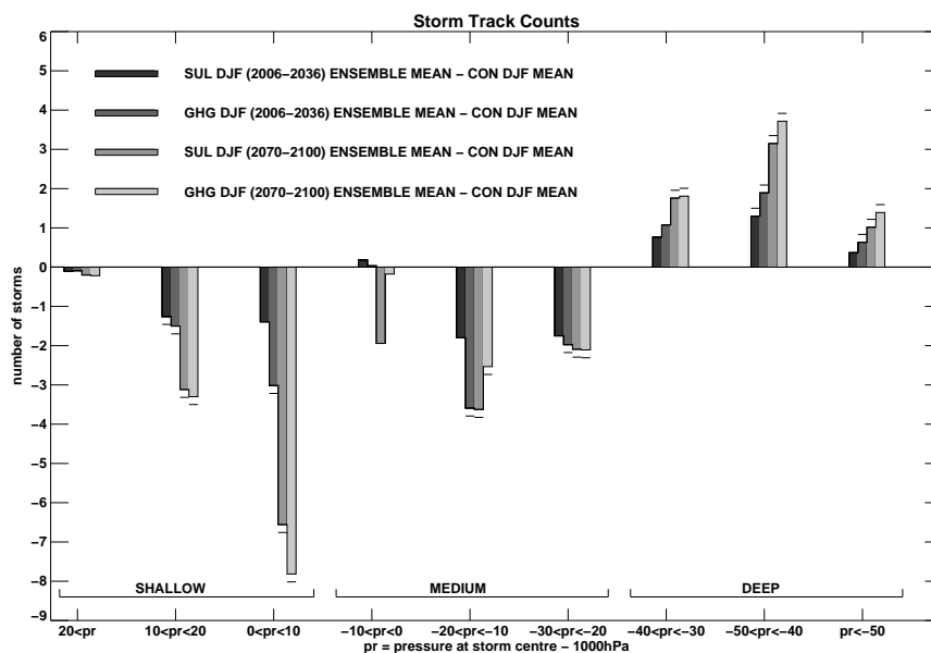
FIG. 7. Number of storm tracks per 90 day December-January-February season in each central pressure band (pr, pressure at storm centre - 1000 hPa). Dark, medium dark, medium light, and light shadings (1st, 2nd, 3rd and 4th peak from left of each group) show the change in the number of storms (relative to the control experiment) in the experiment forced by both greenhouse gases and the direct effect of aerosols (SUL) or by only greenhouse gases (GHG) for two different time periods. Horizontal bars at the end of peaks show changes that are significant at the 1% level. From Carnell and Senior (1998).
