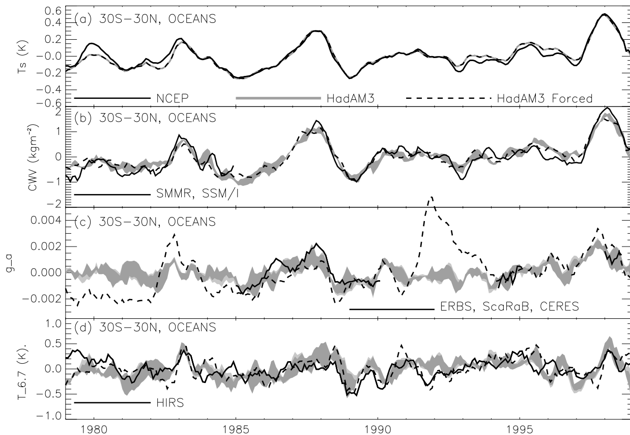
FIG. 14. Interannual variations in (a) surface temperature, (b) column integrated water vapor, (c) atmospheric normalized greenhouse trapping and (d) 6.7 \mu\text{m} brightness temperature for sea surface temperature (SST) forced model (shaded), model with all known forcings (dashed) and observations (solid). Substantial differences between SST only forced experiments and "full forcing" experiments in (c) indicate that the model normalized greenhouse effect is very sensitive to the input of volcanic aerosols and changes in greenhouse gases. From Allan et al. (2003).
