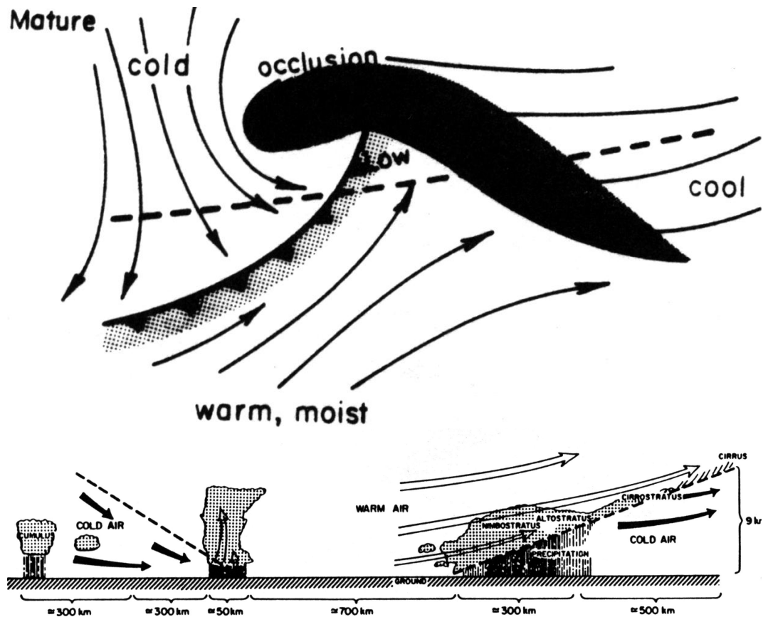
FIG. 5. (top) Schematic of a mature extratropical cyclone represented in the horizontal plane. Shaded areas are regions of precipitation. From Cotton (1990) . (bottom) Schematic vertical cross section through an extratropical cyclone along the dashed line reported on the top figure showing typical cloud types and precipitation. From Cotton (1990), after Houze and Hobbs (1982) .
