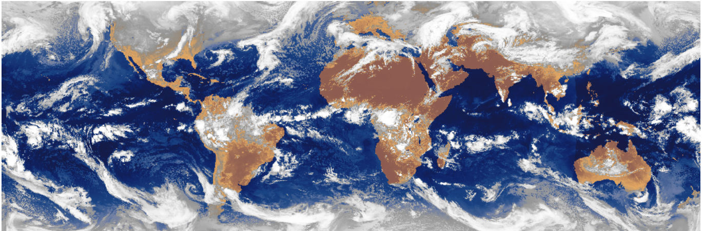
FIG. 2. Composite of instantaneous infrared imagery from geostationary satellites (on March 29th 2004 at 12:00 GMT) showing the contrast between the large-scale organization of the atmosphere and of the cloudiness in the tropics and in the extratropics. From SATMOS (©METEO-FRANCE and Japan Meteorological Agency).
