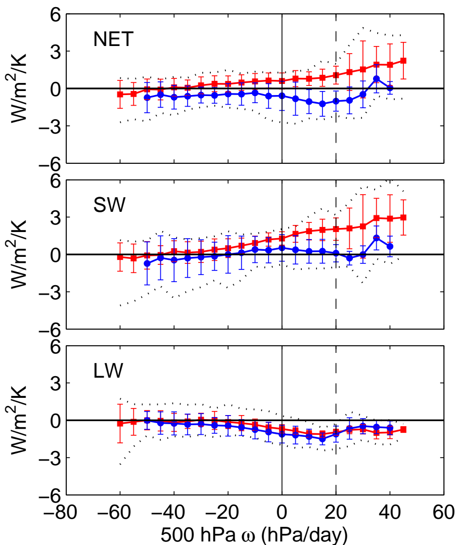
FIG. 10. Sensitivity (in Wm^{-2}K^{-1} ) of the tropical ( 30^{\circ}S-30^{\circ}N ) NET, SW and LW cloud radiative forcing to sea surface temperature changes associated with climate change (in a scenario in which the CO_2 increases by 1% per year) derived from 15 coupled ocean-atmosphere GCMs participating in the AR4. The sensitivity is computed for different regimes of the large-scale atmospheric circulation (the 500 hPa large-scale vertical pressure velocity is used as a proxy for large-scale motions, negative values corresponding to large-scale ascent and positive values to large-scale subsidence). Results are presented for two groups of GCMs: models that predict a positive anomaly of the tropically averaged NET CRF in climate change (in red, 8 models) and models that predict a negative anomaly (in blue, 7 models). From Bony and Dufresne (2005).
