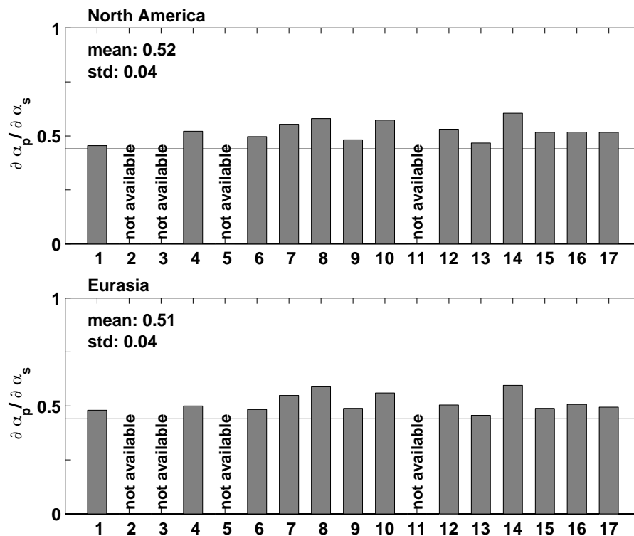
FIG. 18. The dependence of planetary albedo on surface albedo in North American (top) and Eurasian (bottom) land masses poleward of 30^\circ N during northern hemisphere spring, when snow albedo feedback is strongest. Shown with solid horizontal lines are values calculated for the satellite-based ISCCP data set, covering the 1984-2000 period. Shown with grey bars are values based on the 20 th century portion of the transient climate change experiments of the AR4 assessment. This shows how large a typical planetary albedo anomaly is for a 1% surface albedo anomaly. In observations, and in all climate simulations, planetary albedo anomalies are consistently about half as large as their associated surface albedo anomalies. Values are available only for 13 of the 17 experiments because 4 of them do not provide all variables required for the calculation. From Qu and Hall (2005b).
