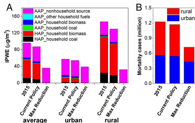
Fig. 5. The impact of replacing household solid fuels with clean energy on IPWE (A) and premature mortality (B) in China. “Current Policy” denotes a scenario in which the official work plan released in 2017 was realized, and “Max Reduction” is a scenario in which all household solid fuels were substituted by electricity and natural gas.
