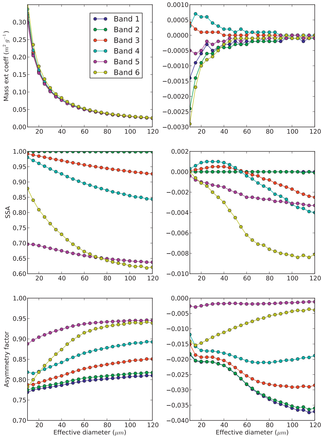
FIG. 1. (top) Mass extinction coefficient, (middle) single-scattering albedo, and (bottom) asymmetry factor as a function of effective diameter for (left) the Fu-Liou model solar bands for severely roughened ice particles. (right) Corresponding differences between the severely roughened and the smooth ice models. The six bands shown correspond to the Fu-Liou RTM SW bands in Table 1.
