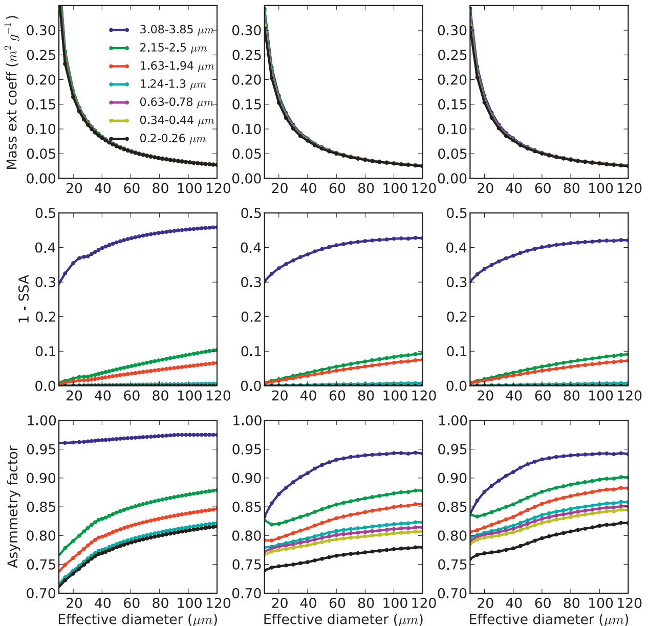
FIG. 5. (top) Mass extinction coefficient, (middle) single-scattering albedo, and (bottom) asymmetry factor as a function of ice particle effective diameter for selected bands in the RRTMG code for (left) the default CAM5 ice cloud model, (middle) the SR ice particle model, and (right) the CS model.
