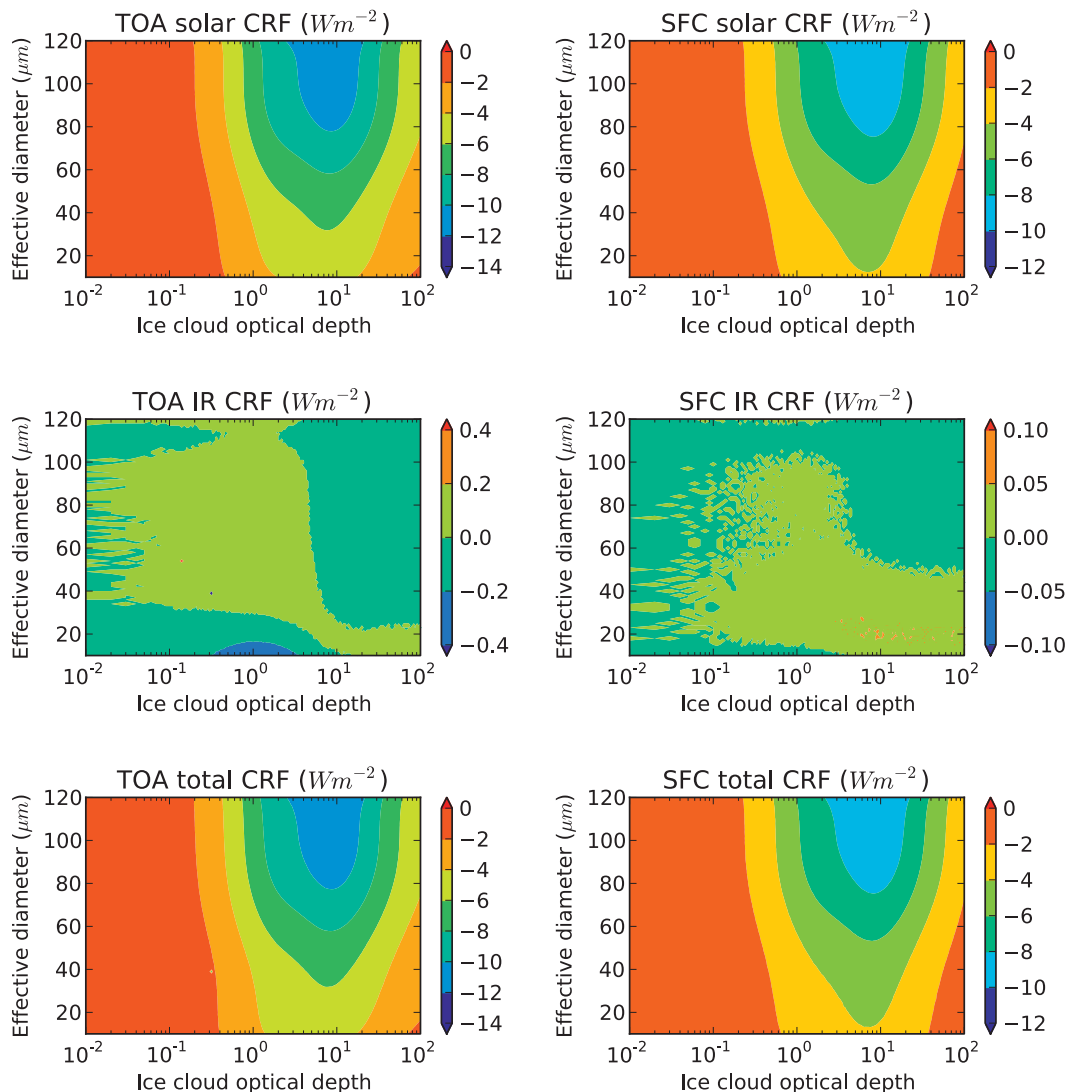
FIG. 3. Ice particle surface roughness effect on (top) SW, (middle) LW, and (bottom) total CRF at SZA = 60^\circ as a function of effective diameter and cloud optical thickness for the Fu–Liou RTM at (left) the TOA and (right) the SFC.
