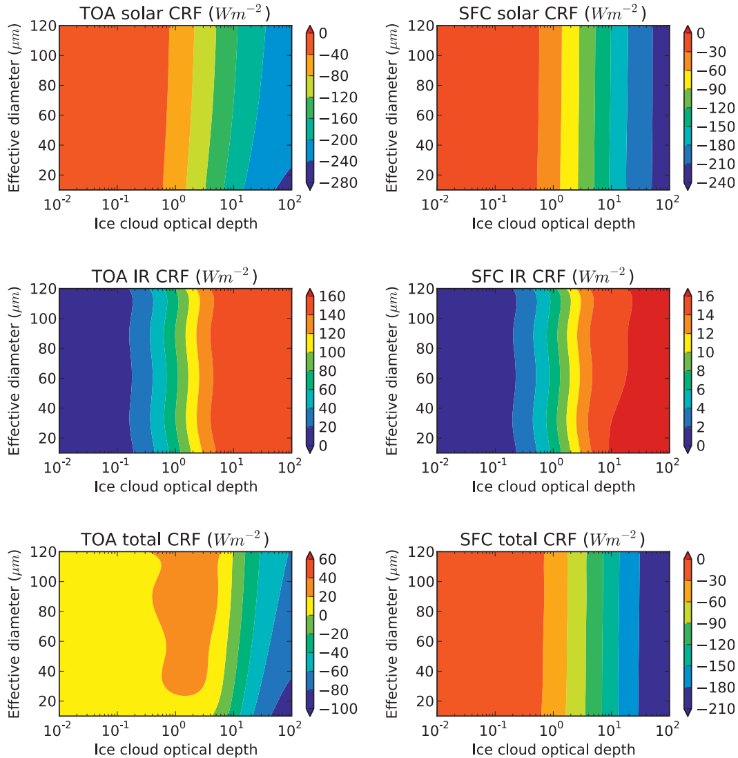
FIG. 2. (top) SW, (middle) LW, and (bottom) total cloud radiative forcing (CRF) at solar zenith angle (SZA) = 60^\circ as a function of effective diameter and cloud optical thickness as simulated by the Fu–Liou RTM for SR ice particles at (left) the TOA and (right) the SFC.
