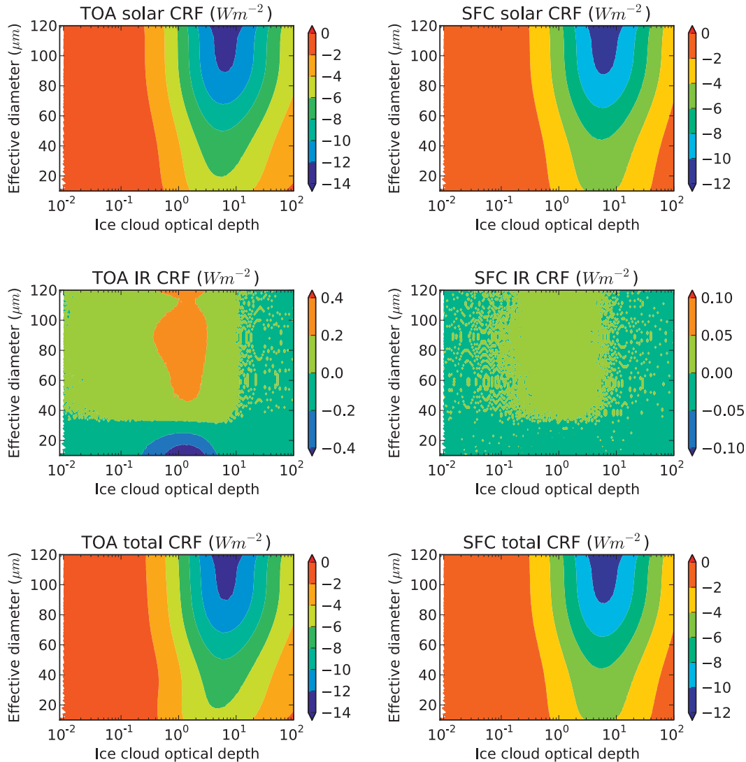
FIG. 4. As in Fig. 3, but for the RRTMG RTM.
