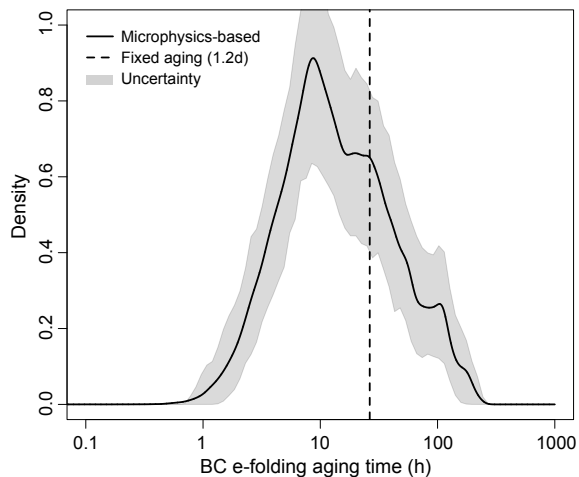
Figure 3. Probability density function of simulated annual mean BC e -folding aging time (h) over the globe for a microphysics-based scheme (solid line) and a fixed aging scheme (dashed line). Also shown is the 95 % uncertainty range (in grey) of the microphysics-based aging time estimated from a Monte Carlo method.
