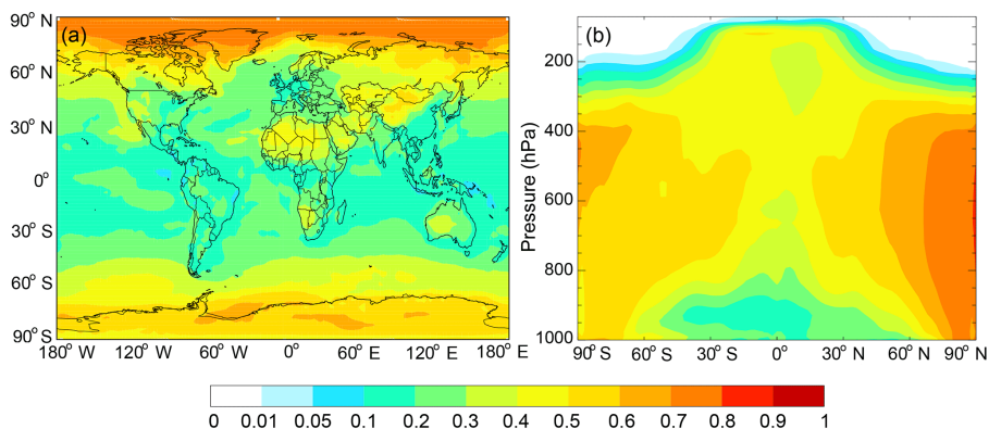
Figure 10. GEOS-Chem simulated annual mean contribution of chemical oxidation to the total BC aging rate (sum of condensation, coagulation, and chemical oxidation) averaged within 0–1 km above the surface (left) and zonally (right). Model results are for 2009.
