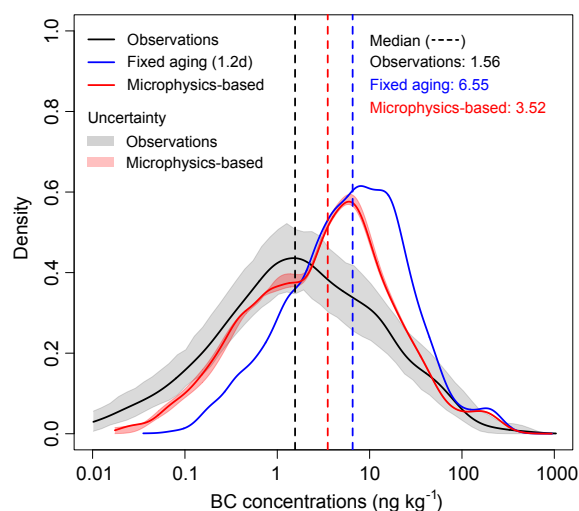
Figure 5. Probability density functions of HIPPO observed (black) and GEOS-Chem simulated BC concentrations. Model results using a fixed BC aging (blue) and a microphysics-based aging (red) are shown. The 95 % uncertainty range of the HIPPO observations, estimated from a Monte Carlo method, is shown (in grey). Also shown (in light red) is the range of model results from microphysics-based sensitivity simulations (see Table 1 and text for details). Dashed lines show the median of observations ( 1.56 \text{ ng kg}^{-1} , black), fixed aging ( 6.55 \text{ ng kg}^{-1} , blue), and microphysics-based aging ( 3.52 \text{ ng kg}^{-1} , red). About 5 % of the observed BC concentrations are below 0.01 \text{ ng kg}^{-1} .
