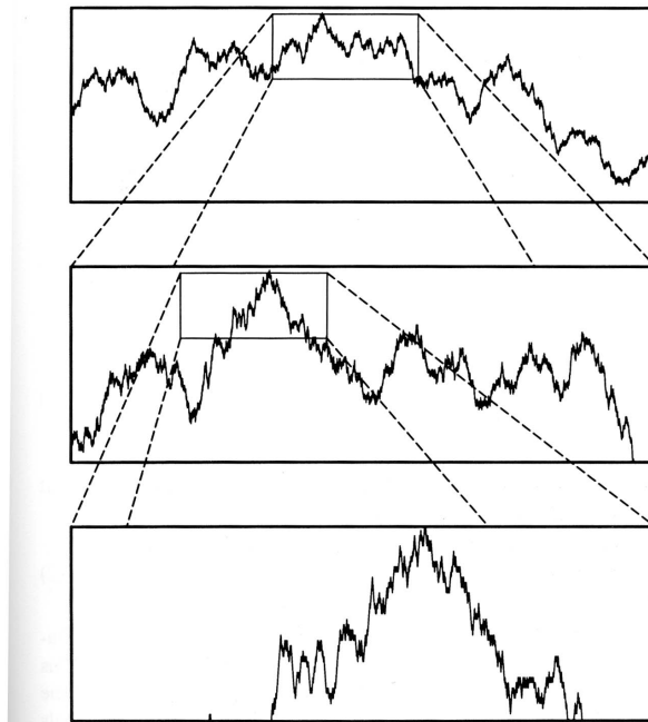
Figure 6: Brownian motion: a portion of a time series y(t) for a random velocity increment v(t)dt , enlarged twice, illustrating its self-similarity ( i.e. , scale invariance). (Frisch, 1995)
