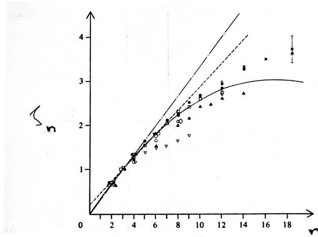
Figure 9: Variation of exponent \zeta_n as a function of the order n from different experiments with different Re values. The curves are various model fits: the dash-dot line is from Kolmogorov (1941); the dashed line is the \beta model of Frisch et al. (1978), and the solid line is from a log-normal distribution. (Anselmet et al. , 1984)
