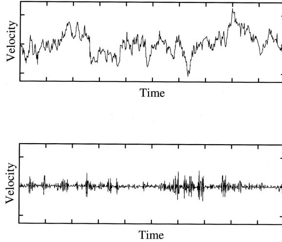
Figure 7: (Top) Velocity signal from a jet with Re_\lambda \approx 700 . (Bottom) Same signal as in (a) subject to high-pass filtering showing intermittent bursts. (Gagne, 1980)
