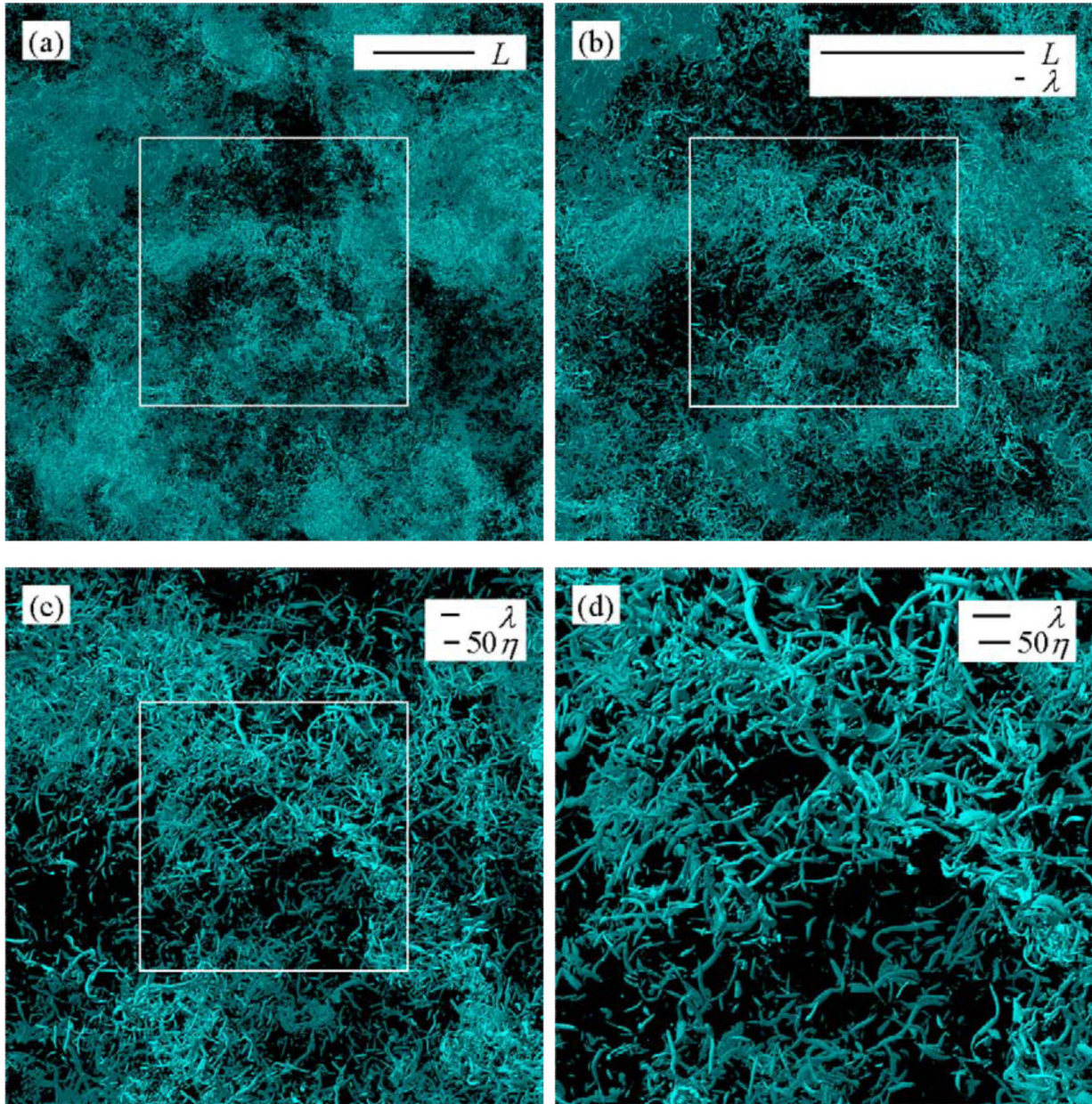
Figure 14: |\zeta| iso-surfaces at several magnifications in a computational simulation of randomly forced, 3D, isotropic, homogeneous turbulence. (L, \lambda, \eta) = forcing, Taylor, and Kolmogorov scales. (Kaneda, 2005)
